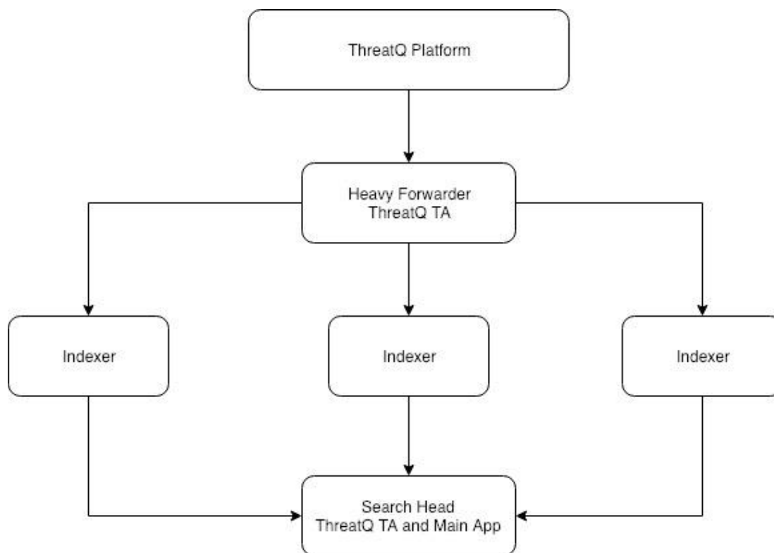
Figure 3: Deployment of Splunk App in Distributed Environment
